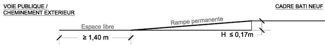
Figure 8.1 – Coupe verticale
